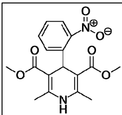
Figure 4-6: Chemical Structure of Nifedipine
