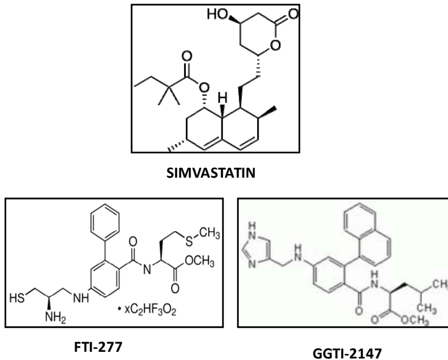
Figure 6-2: Chemical structures of inhibitors of protein prenylation
