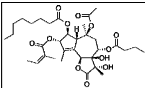
Figure 4-1: Chemical Structure of Thapsigargin
